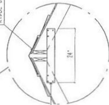
PEAK CONNECTION DETAIL
